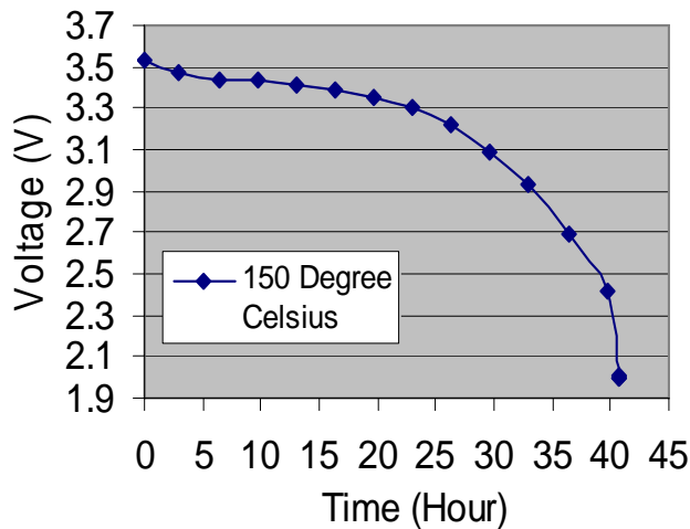
High Temperature Discharge(325mA)
