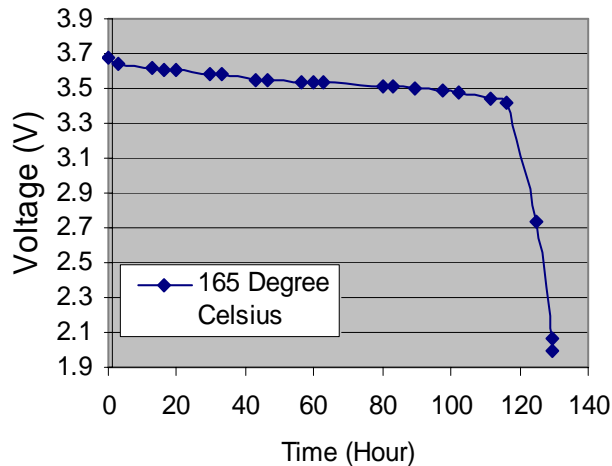
High Temperature Discharge(50mA)
